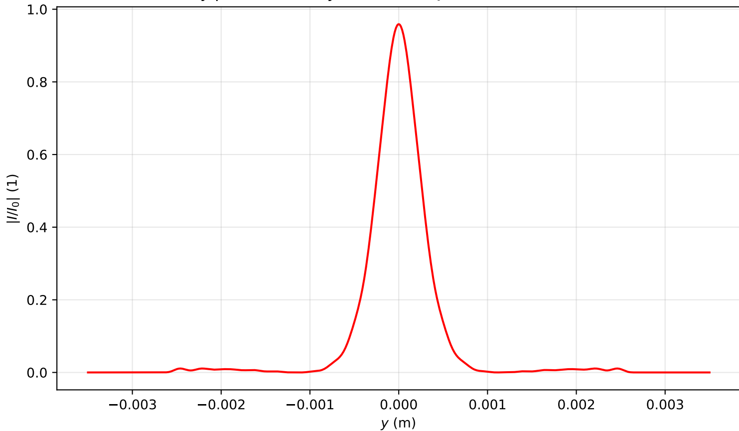
Intensity profile I(x=0, y, z=1.592)/I_0 , P_{in}=1.0P_{cr} , artificial time
